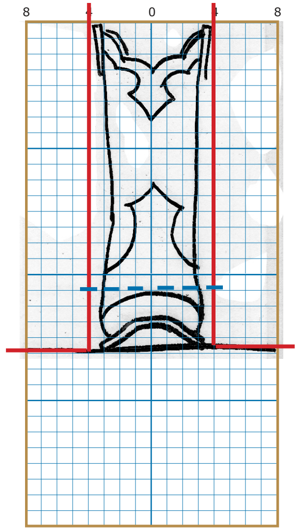
SIDE VIEW
